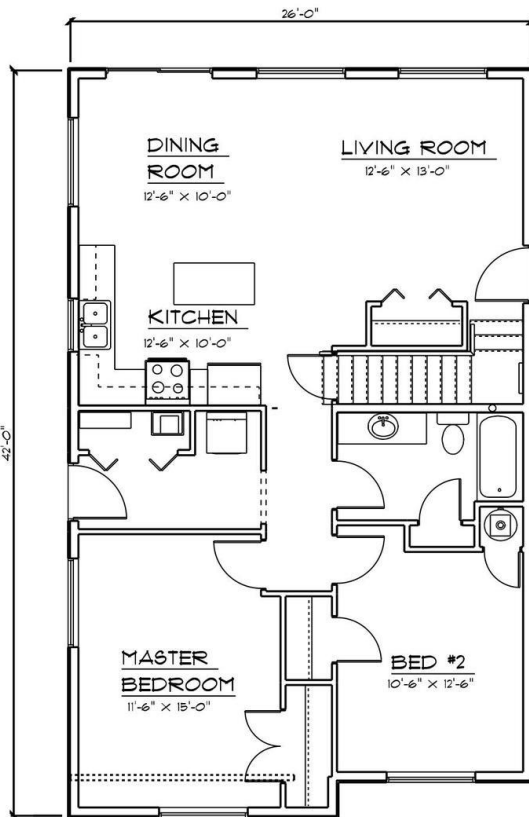
MAIN FLOOR PLAN 1070 SQ FT
